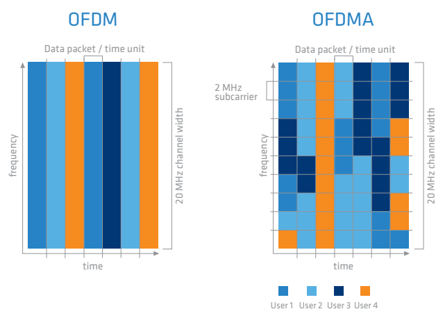
Fig. 1: OFDM (Wi-Fi 5) compared with OFDMA (Wi-Fi 6) technology
